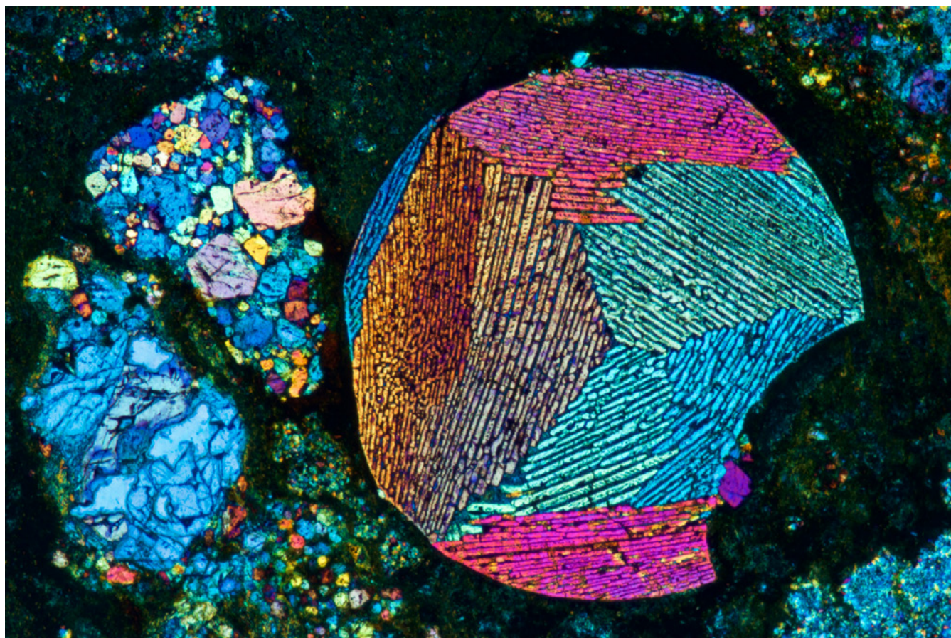
Figure 6. Cross polarized nicols image of a chondritic meteorite. It is to be noted the barred olivine chondrule on the right-middle of the image. Museum of Planetary Sciences – Prato, Italy. Photo credit Prof. Bernardo Cesare (University of Padova).
